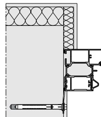
Blockzarge Ankermontage
