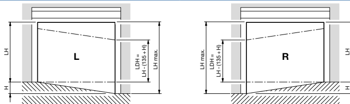
Chamfered bottom profile – view of fitting side Internal roller garage door from inside External roller garage door from outside
